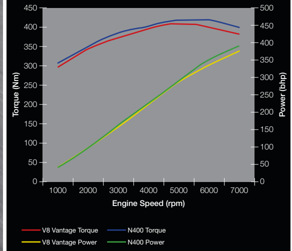
POWER AND TORQUE CURVE
